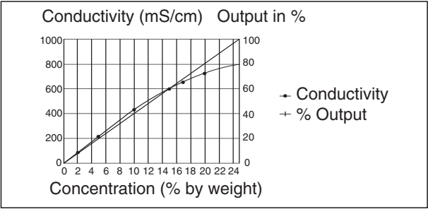
Linearisation of output Example: 0-25% Sulfuric acid
